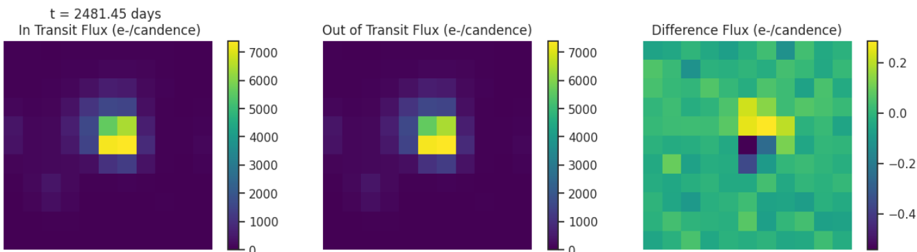
Fig 6. Difference images for target TIC 172219408 for each transit like event. Left: mean in-transit flux(left). Middle: mean out-of-transit flux. Right: difference between the mean out-of-transit and mean in-transit flux. Ensure that the change in brightness occurs on target.
