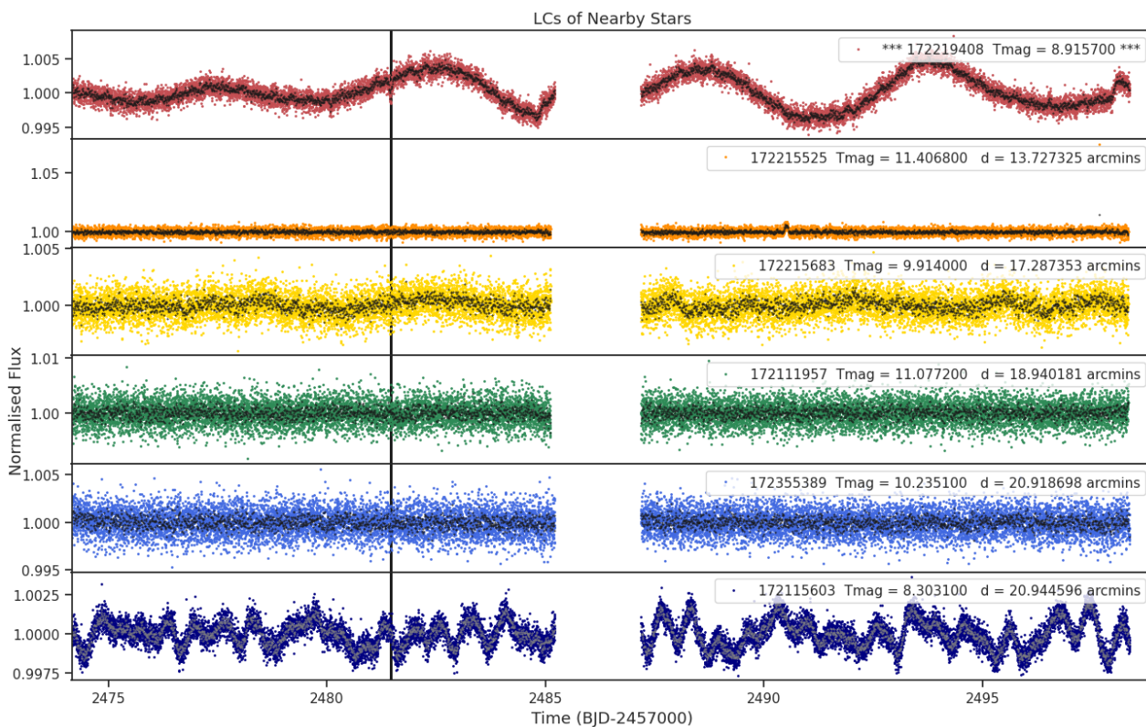
Fig 8. Lightcurves of the five closest stars to target 172219408 (top panel). The distances to the target star and the TESS magnitudes are shown for each star. Only ever shown for one sector.
