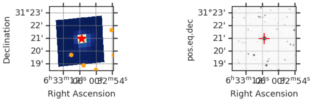
Fig 7. The locations of nearby GAIA DR2 stars with a magnitude difference less than 5 (orange circle) within the TESS Cut Out around TIC 172219408 (red star). Only shown for one sector. Right: SDSS image of the surrounding field.
