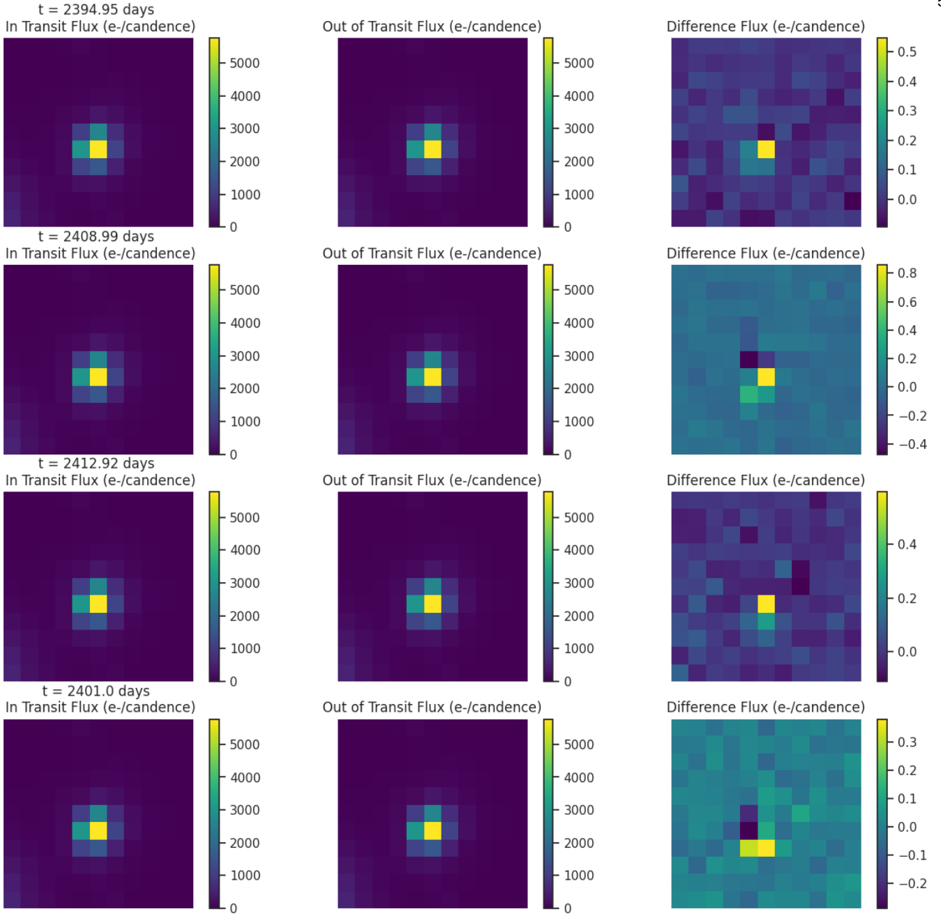
Fig 6. Difference images for target TIC 155639758 for each transit like event. Left: mean in-transit flux(left). Middle: mean out-of-transit flux. Right: difference between the mean out-of-transit and mean in-transit flux. Ensure that the change in brightness occurs on target.
