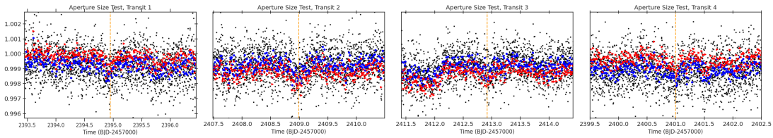
Fig 4. The lightcurve around the time of each transit-like event extracted with the SPOC pipeline defined aperture (binned:blue, unbinned:grey) and the with an aperture that is 40 per cent smaller (red). The flux is extracted from the target pixel files (TPFs) and has not been detrended or corrected for systematics. The vertical orange line indicates the time of the transit-like event.
