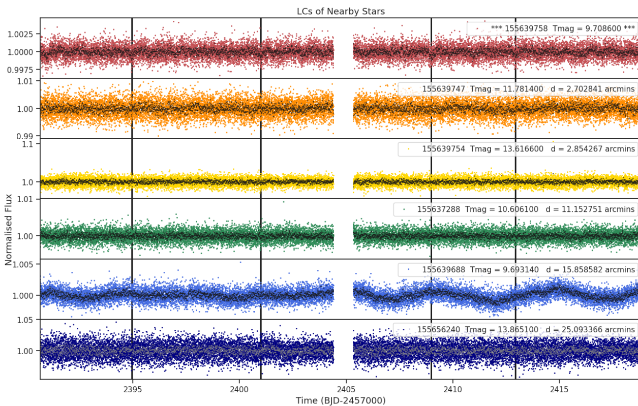
Fig 8. Lightcurves of the five closest stars to target 155639758 (top panel). The distances to the target star and the TESS magnitudes are shown for each star. Only ever shown for one sector.
