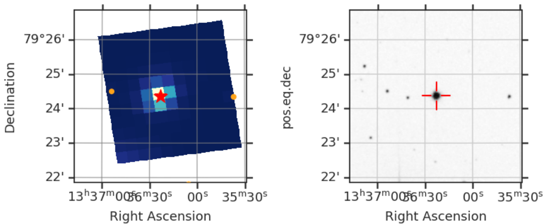
Fig 7. The locations of nearby GAIA DR2 stars with a magnitude difference less than 5 (orange circle) within the TESS Cut Out around TIC 155639758 (red star). Only shown for one sector. Right: SDSS image of the surrounding field.
