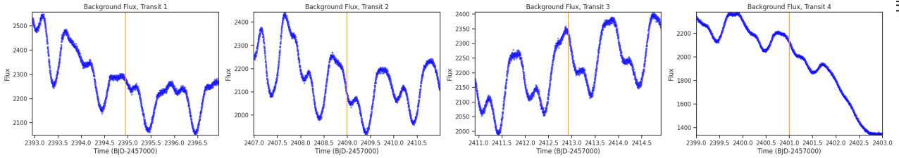
Fig 2. Background flux vs. time around the time of each transit-like event. The vertical orange line indicates the time of the transit-like event.
