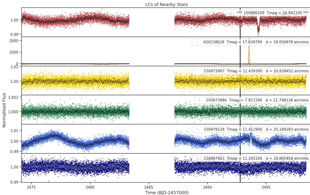
Fig 8. Lightcurves of the five closest stars to target 150986109 (top panel). The distances to the target star and the TESS magnitudes are shown for each star. Only ever shown for one sector.
