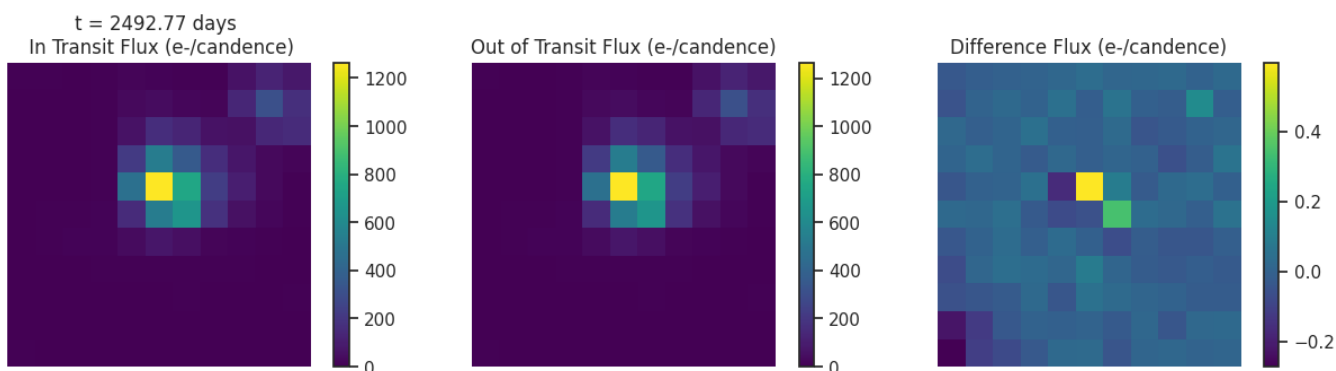
Fig 6. Difference images for target TIC 150986109 for each transit like event. Left: mean in-transit flux(left). Middle: mean out-of-transit flux. Right: difference between the mean out-of-transit and mean in-transit flux. Ensure that the change in brightness occurs on target.
