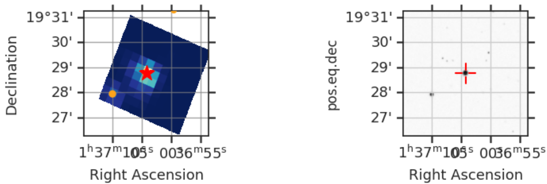
Fig 7. The locations of nearby GAIA DR2 stars with a magnitude difference less than 5 (orange circle) within the Tess Cut Out around TIC 150986109 (red star). Only shown for one sector. Right: SDSS image of the surrounding field.
