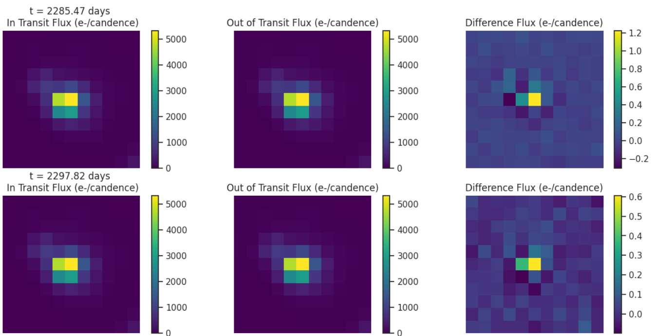
Fig 6. Difference images for target TIC 142146051 for each transit like event. Left: mean in-transit flux(left). Middle: mean out-of-transit flux. Right: difference between the mean out-of-transit and mean in-transit flux. Ensure that the change in brightness occurs on target.
