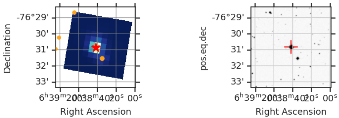
Fig 7. The locations of nearby GAIA DR2 stars with a magnitude difference less than 5 (orange circle) within the Tess Cut Out around TIC 142146051 (red star). Only shown for one sector. Right: SDSS image of the surrounding field.
