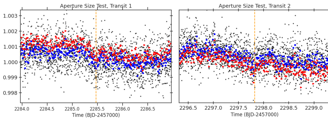
Fig 4. The lightcurve around the time of each transit-like event extracted with the SPOC pipeline defined aperture (binned:blue, uninned:grey) and the with an aperture that is 40 per cent smaller (red). The flux is extracted from the target pixel files (TPFs) and has not been detrended or corrected for systematics. The vertical orange line indicates the time of the transit-like event.
