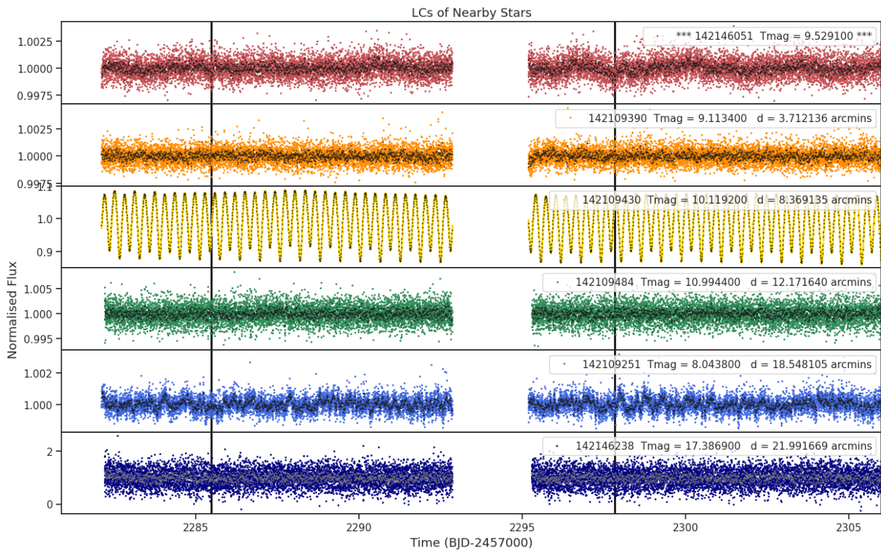
Fig 8. Lightcurves of the five closest stars to target 142146051 (top panel). The distances to the target star and the TESS magnitudes are shown for each star. Only ever shown for one sector.
